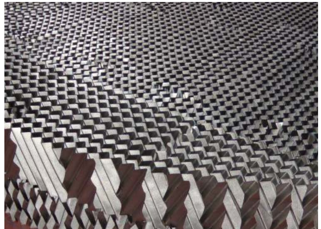
Baretti Structured Packing
